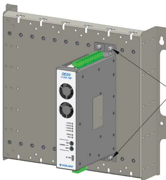
Mount Amplifier Module with four M6 x 10 Screws provided with module.
